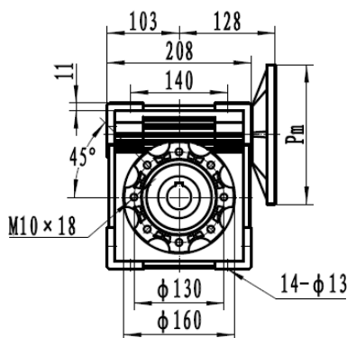
Input shaft hole
